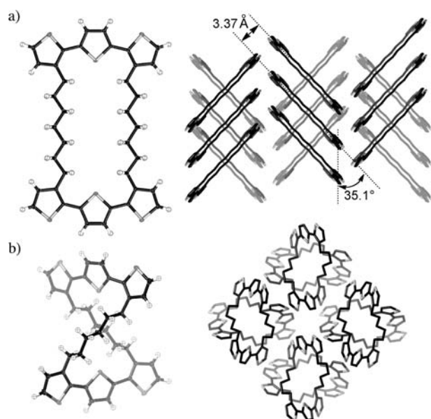
Figure 2. X-ray crystal structures of a) 1 and b) 2 : molecular structure (left) and crystal packing (right). Ellipsoids set at 50% probability; C black, S gray, H white.
